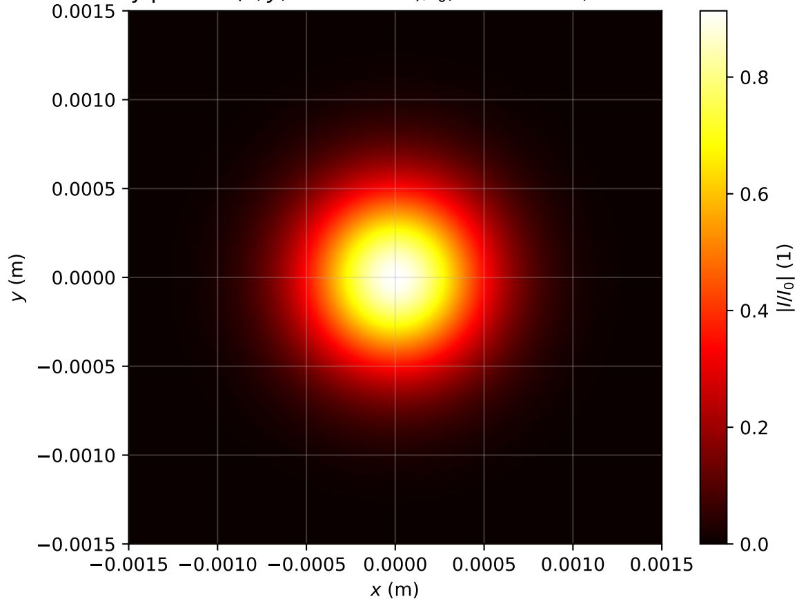
Intensity profile I(x, y, z = 0.876m)/I_0 , P_{in}=0.2P_{cr} , artificial time
